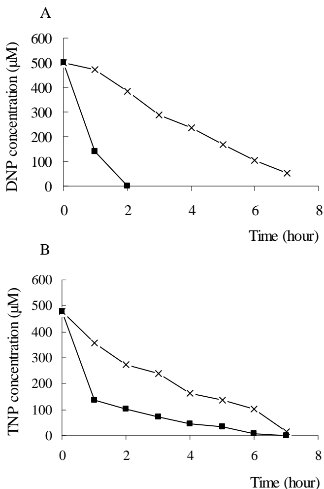
Fig.13. Transformation of DNP (A) or TNP (B) by resting cells of R. opacus HL PM-1 (x) and R. opacus ND1 (■). The cultures were harvested at the mid-log phase and resuspended in \text{KH}_2\text{PO}_4/\text{K}_2\text{HPO}_4 buffer (50 mM, pH 7.5) supplemented with 0.5 mM DNP or TNP. \text{OD}_{600\text{nm}} of the cell suspensions after resuspension was 1.7-1.8. The samples were collected at relevant time intervals and analysed by HPLC as described in Materials and Methods. The values are the average values of two independent experiments.
