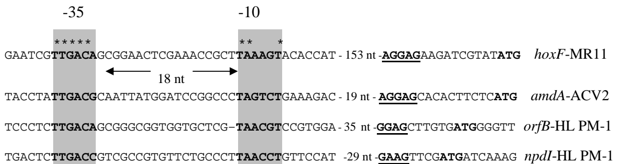
Fig.28. Sequence comparison of the promoter regions from npd operons showing the -35 and -10 hexamers. Top: promoter sequence of the hydrogenase gene cluster from R. opacus MR11 ( hoxF gene encoding the alpha subunit of the hydrogenase, Genbank U70364). Second from top: upstream sequence of the amdA-nthAB genes from Rhodococcus sp. ACV2 ( amdA gene encoding the amidase protein Z48769). Third from top: upstream sequence of the orfB gene from R. opacus HL PM-1. Bottom: upstream sequence of the npdI gene from R. opacus HL PM-1 (Genbank AF323606). Boxes indicate conserved -35 and -10 regions; putative Shine-Dalgarno sequences are indicated by bold type and underlining; translation start codons are indicated by bold type.
