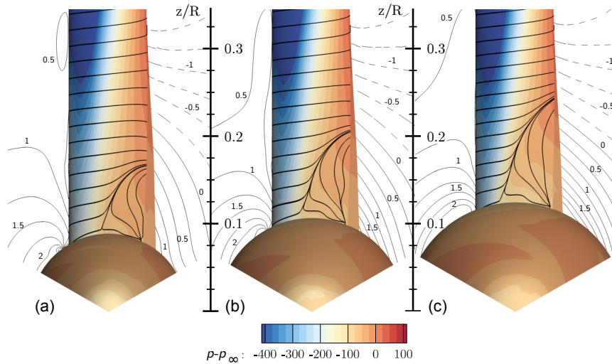
Figure 16. Visualization of three-dimensional flow in the root region using streamlines and pressure contours for CaseT1.0 (a), CaseT1.2 (b) and CaseT1.4 (c). The contour lines are plotted for a slice at x = 2 m and indicate the velocity \tilde{w} = w - \Omega y , which denotes the deviation from the ideal kinematic path.
