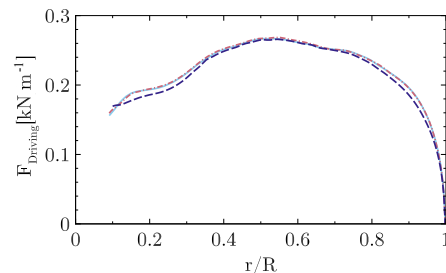
Figure B3. Influence of boundary layer transition on the sectional driving force. Fully turbulent k-\omega -SST (dashed), \gamma-Re_\theta-k-\omega -SST (solid), e^N-k-\omega -SST (dashed dot).
