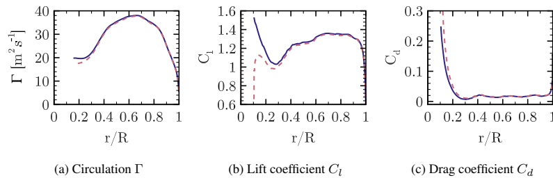
Figure 15. Distribution of aerodynamic coefficients along the blade radius for CaseIsoRotor (dashed) and CaseT1.0 (solid).
