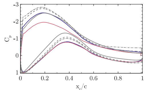
Figure 14. Pressure coefficient C_p at r/R = 0.136 for CaseIsoRotor (solid red) and CaseTI.0 (solid blue) compared with two-dimensional simulations (gray lines): \alpha = 10.2^\circ (solid), \alpha = 13^\circ (dashed), \alpha = 14^\circ (dashed dot).
