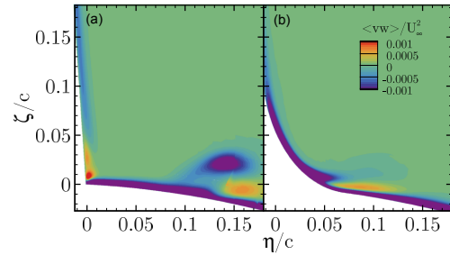
Figure 31. Reynolds shear stress \langle vw \rangle of the chord-wise and span-wise velocity at x_c/c = 0.5 . CaseT1.0 (a), CaseT1.0-fairing (b).
