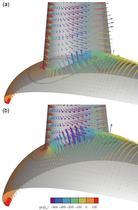
Figure 19. Inviscid pressure distribution in the junction region of the blade and nacelle for CaseT1.0 (a) and CaseT1.4 (b).
