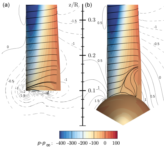
Figure 9. Visualization of three-dimensional flow in the root region using streamlines and pressure contours on the suction side of the blade for CaseIsoRotor (a) and CaseTI.0 (b). The contour lines indicate the “deviation velocity” \tilde{w} from the ideal kinematic value -\Omega y in a slice at x = 2 m.
