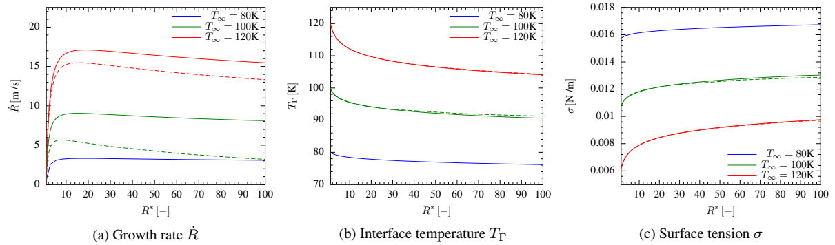
Figure 1. Results from the 1-D solution as function of relative bubble size R^* = R/R_{\text{crit}} for the range of liquid temperatures T_\infty (80 K to 120 K) and pressures p_\infty = 10^3 \text{ Pa} (solid lines) and p_\infty = 10^5 \text{ Pa} (dashed lines).
