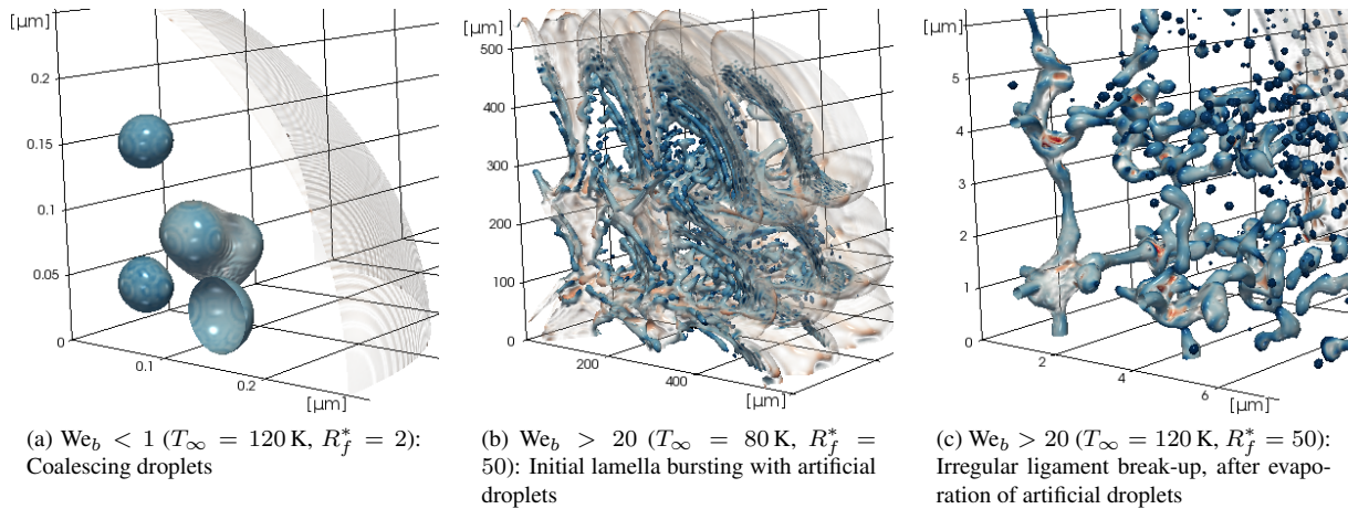
Figure 5. Alternative break-up behaviours found in different test cases
