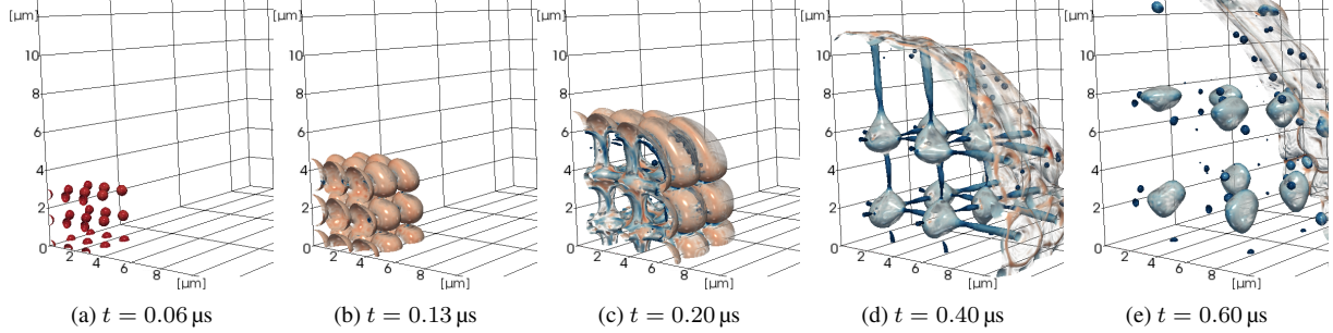
Figure 3. Simulation of bubble growth and liquid break-up for the case p_\infty = 1000 Pa, T_\infty = 100 K, R_f^* = 10 , We_b = 12.6 . Surfaces correspond to the iso-surface of the volume fraction with f = 0.5 . The surface is coloured according to curvature as red for bubbles and blue for droplets.
