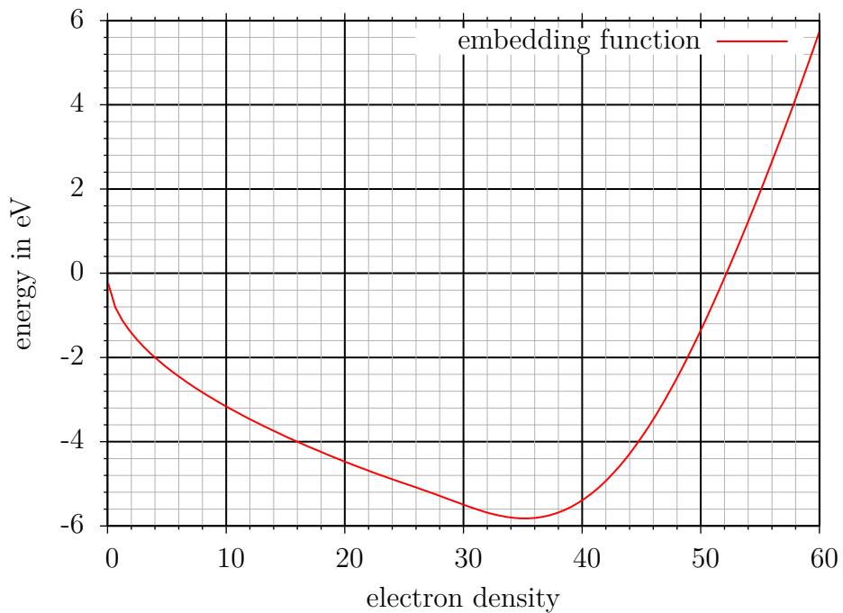
Figure 3.6: Embedding function of the titanium potential
