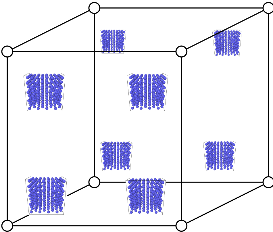
Figure 7.19: Stress free hexahedron, FCC to BCC, subproblems after transition
