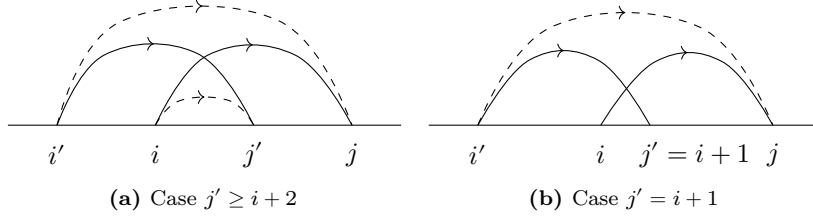
Figure 2: Non-split extensions.
