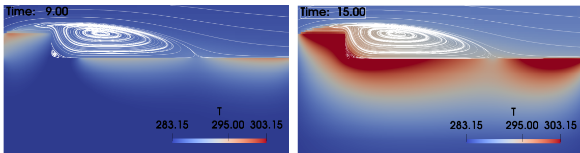
Figure 7.13: Temperature distribution at 9 a.m. and 3 p.m. in the sandy soil.
