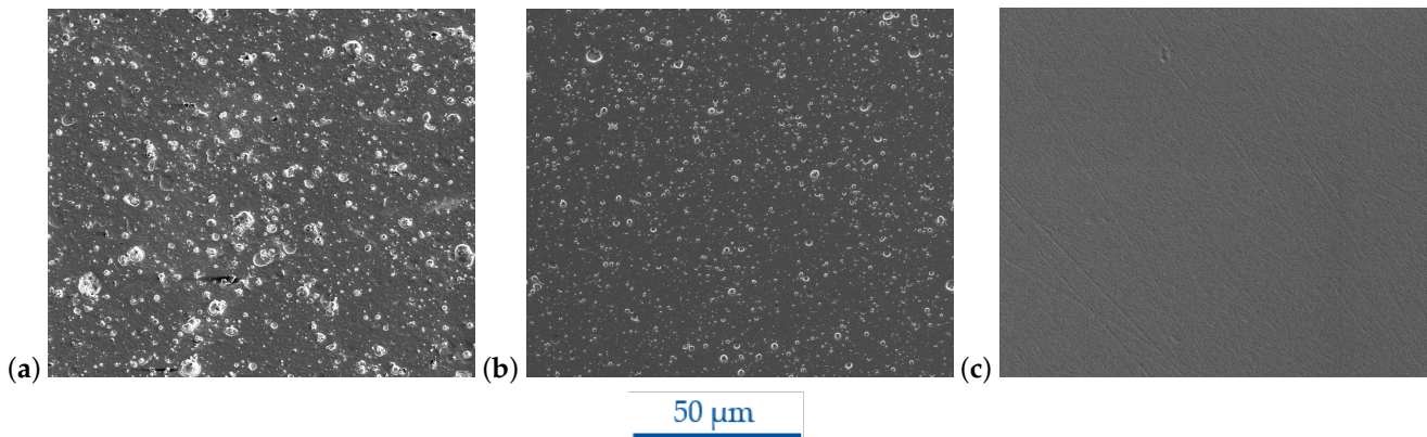
Figure 4. SEM images of CrN coatings provided by different manufacturers; (a) CrN 1 M3, (b) CrN 2 M4 and (c) CrN 3 M1 coating at FOV 128 \mu\text{m} .
