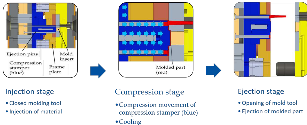
Figure 2. Mold tool and basic injection–compression molding’s processing sequence.
