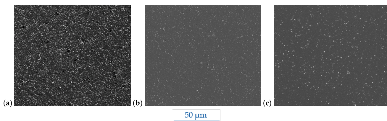
Figure 3. SEM images of tetrahedral hydrogen-free amorphous diamondlike carbon coatings provided by different manufacturers; (a) DLC ta-C 1 M1, (b) DLC ta-C 2 M1 and (c) DLC ta-C 3 M2 coating at FOV 128 \mu\text{m} .
