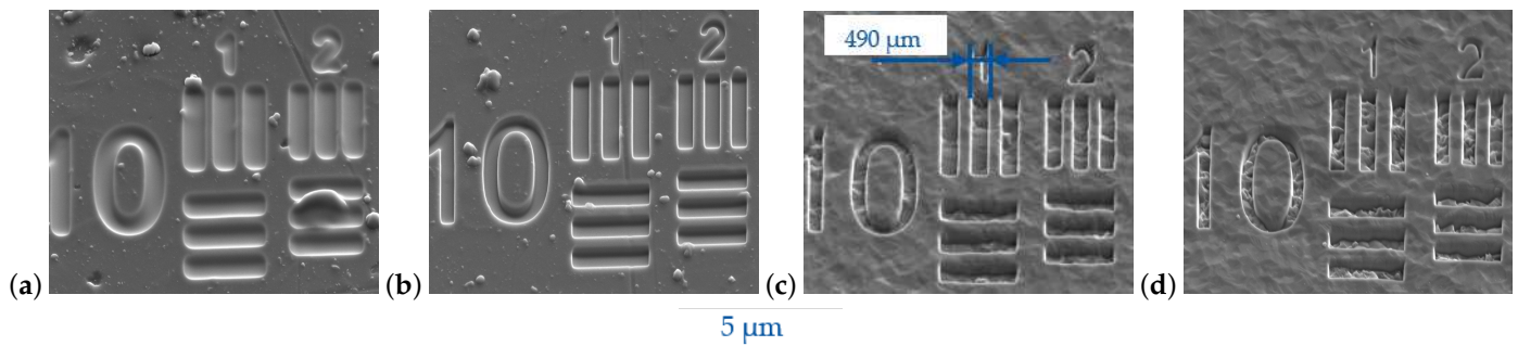
Figure 5. SEM images of USAF group 10 elements 1 and 2 FIB-milled into diamondlike carbon ta-C at beam currents (a) I = 260 pA and (b) I = 9 pA and into HiPIMS CrN at beam currents (c) I = 260 pA and (d) I = 9 pA.
