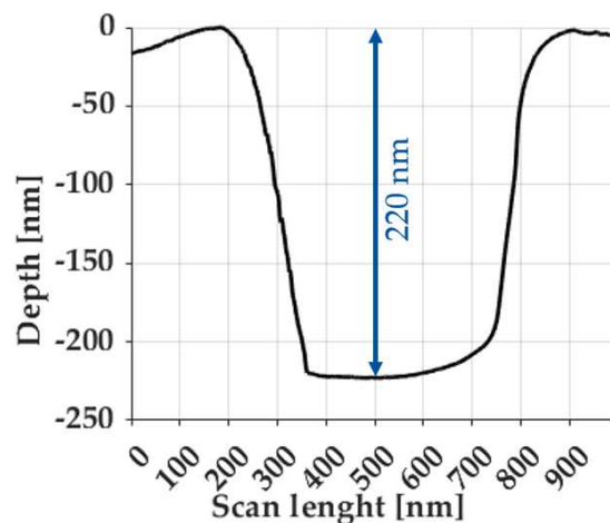
Figure 6. Profile depths of test pattern FIB-milled into CrN.
