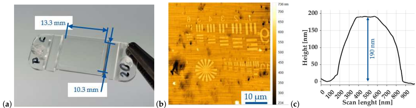
Figure 7. (a) Molded PC LEXAN 133R part with dimensions of the surface area containing replicated features; (b) AFM scan of full test pattern replicated from FIB-milled DLC ta-C hard coating; (c) profile height of replicated USAF 10 group 1 vertical bar onto PC for CrN.
