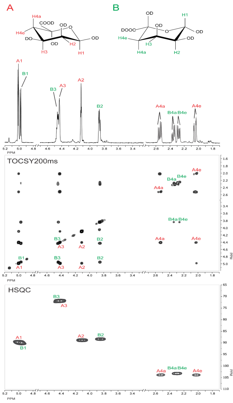
Supplementary Figure S8. 2D TOCSY and HSQC spectra of the cyclic stereoisomers A and B. (see also Figure 8 and Figure 9 in main text). Protons and carbons are assigned according to Enquist et al. (2014).
