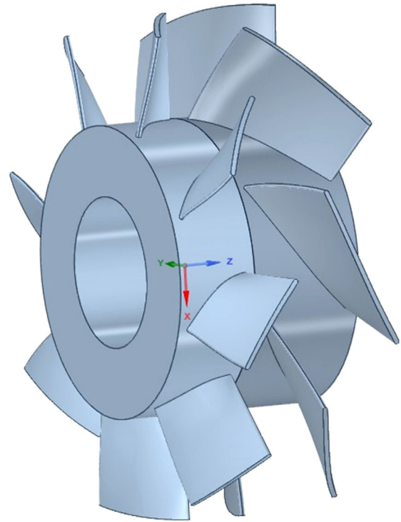
FIGURE 1 Initial Shaft-Driven Contra-rotating Reversible Pump Turbine (SD-CRRPT) design
