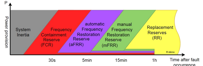
FIGURE 8 Frequency control measures in ENTSO-E area [69]
