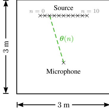
Figure 3.11: Time-varying RIR estimation setup
