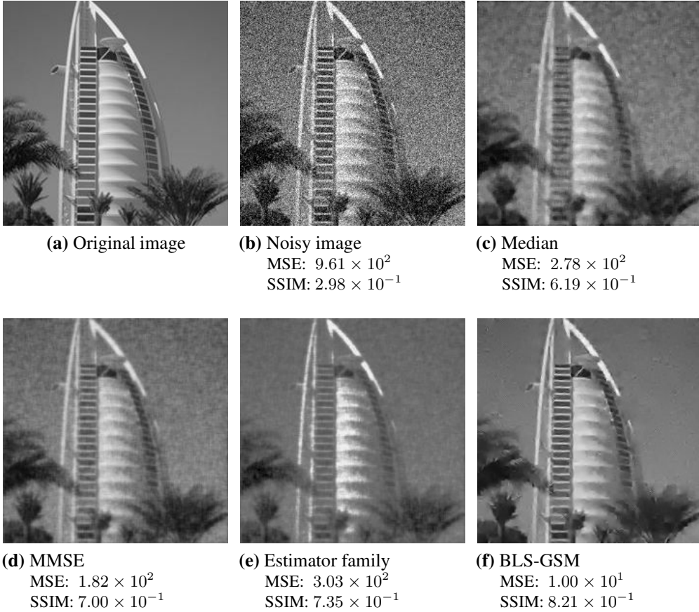
Figure 4.5: Example 3: Results of the various reconstruction methods ( \sigma = 30 )
