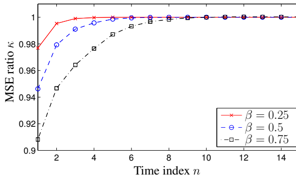
Figure 3.6: Example 1: Ratio of the mean squared errors for RAMX and its steady-state approximation
