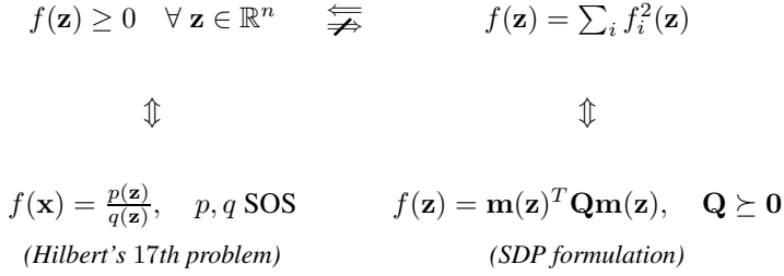
Figure C.2: Relationship between nonnegative polynomials and SOS
