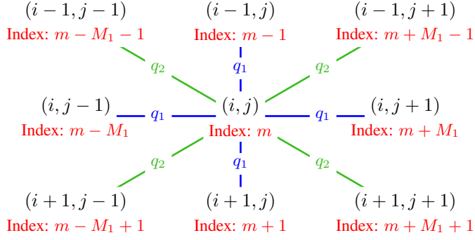
Figure 4.4: Example 3: Nearest neighbour dependency graph at position (i, j) . The corresponding linear index of the pixels with respect to the whole image are given in red.
