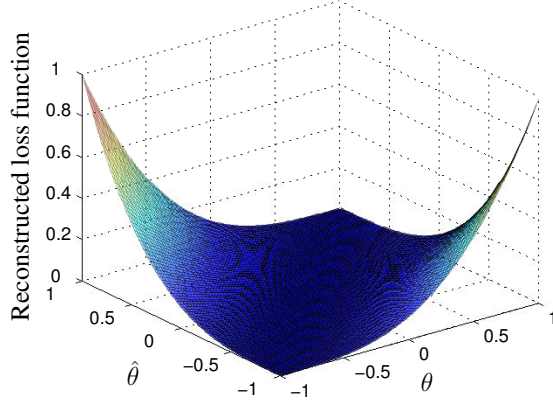
Figure 5.2: Example 1: Reconstructed loss ( D = 3 , unit volume regularization)
