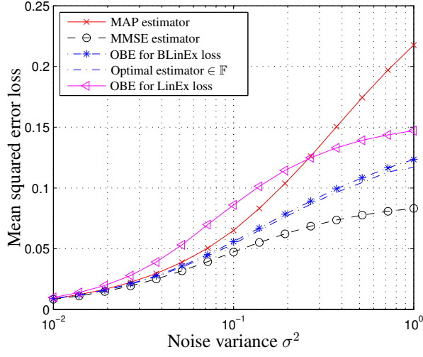
(a) Squared error
