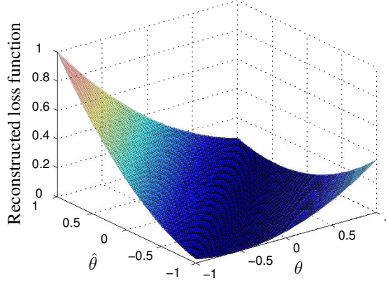
Figure 5.4: Example 2: Reconstructed loss ( D = 1 , unit volume regularization)
