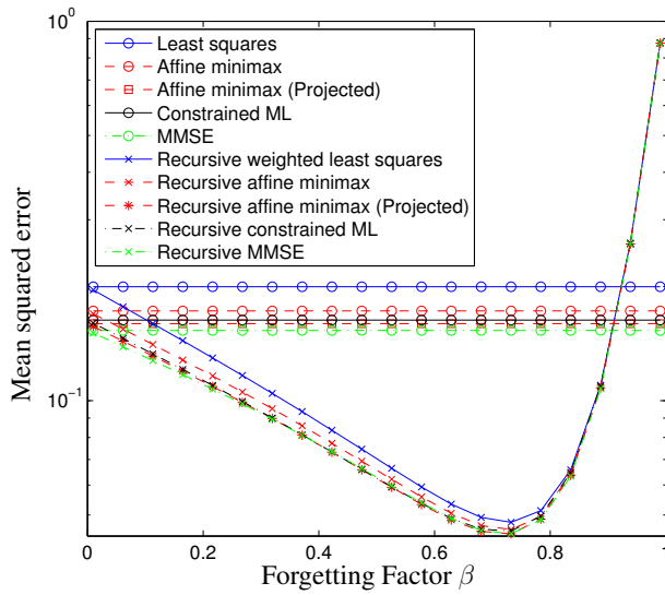
Figure 3.4: Example 1: Mean squared error vs. the forgetting factor \beta for N = 137
