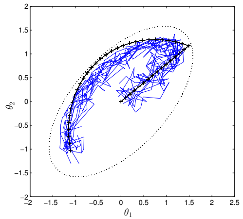
(h) Recursive MMSE
