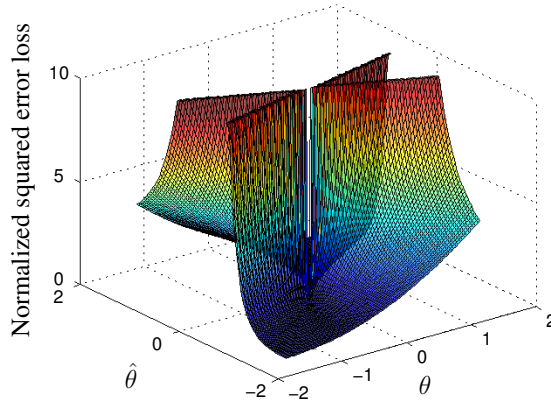
Figure 5.5: Example 3: Normalized squared error loss
