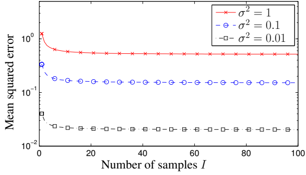
Figure 3.5: Example 1: Mean squared error for varying number of Monte Carlo samples
