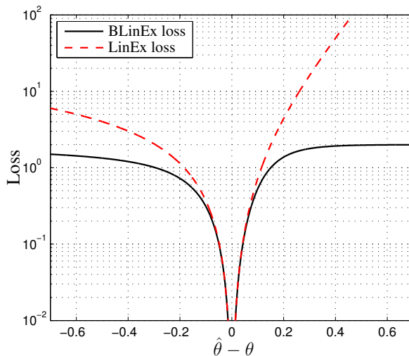
Figure 4.2: Example 1: LinEx and BLinEx loss ( \rho = 0.5 , a = 10 and b = 1 )
