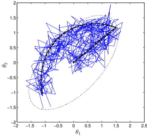
(e) Affine minimax
