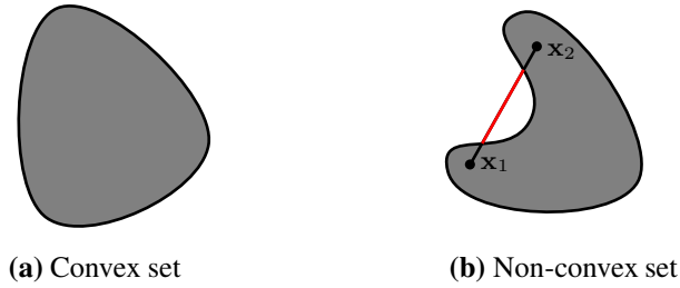
Figure B.1: Example of a convex and non-convex set
