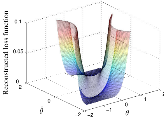
Figure 5.6: Example 3: Reconstructed loss ( D = 5 , unit volume regularization)
