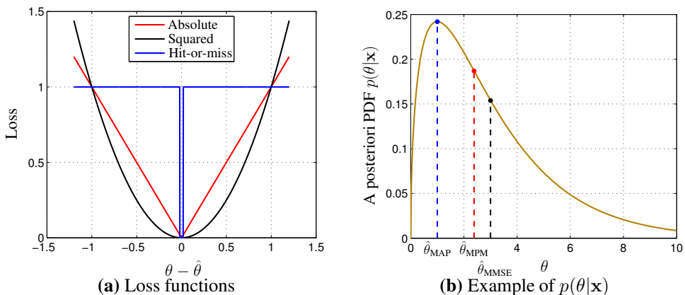
Figure 2.1: Comparison of the MPM, MMSE and MAP estimator
