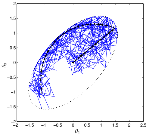
(c) Constrained ML
