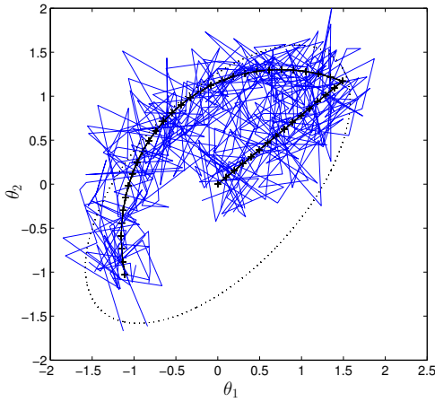
(a) Weighted least squares
