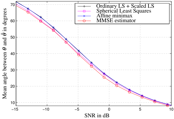
Figure 3.10: Example 2, Case B: Comparison of averaged angle in degrees
