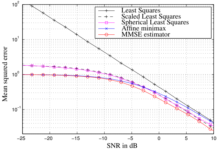
Figure 3.9: Example 2, Case B: Comparison of averaged squared error
