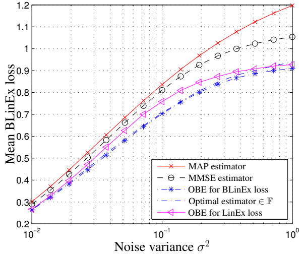
(b) BLinEx loss
