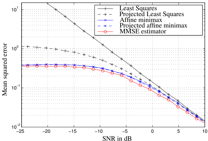
Figure 3.7: Example 2, Case A: Comparison of averaged squared error
