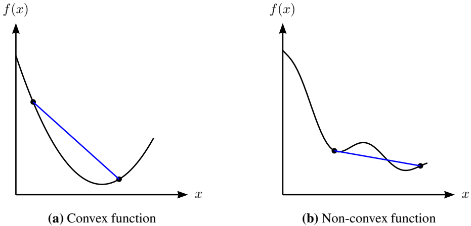
Figure B.2: Example of a convex and non-convex function
