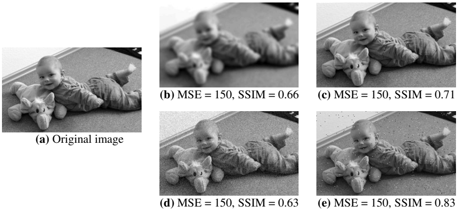
Figure 4.1: Comparison of MSE with SSIM for different image operations (b) = Gaussian blurring with \sigma = 2.27 , (c) = image rotation by \beta = 0.7^\circ , (d) = additive uniform noise, (e) = salt and pepper noise
