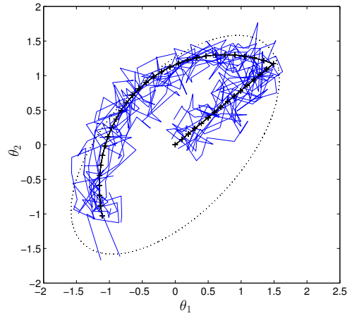
(b) Recursive weighted least squares
