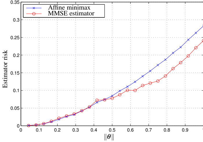
Figure 3.8: Example 2, Case A: Comparison of estimator risk
