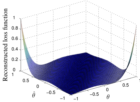
Figure 5.3: Example 1: Reconstructed loss ( D = 3 , trace regularization)
