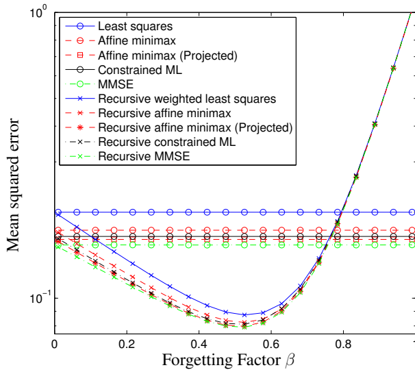
Figure 3.3: Example 1: Mean squared error vs. the forgetting factor \beta for N = 45
