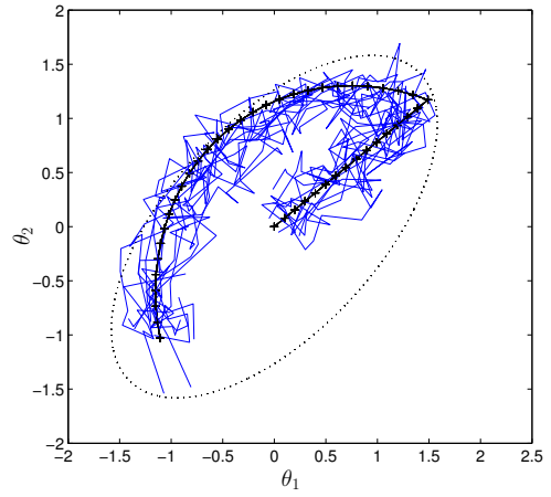
(f) Recursive affine minimax
