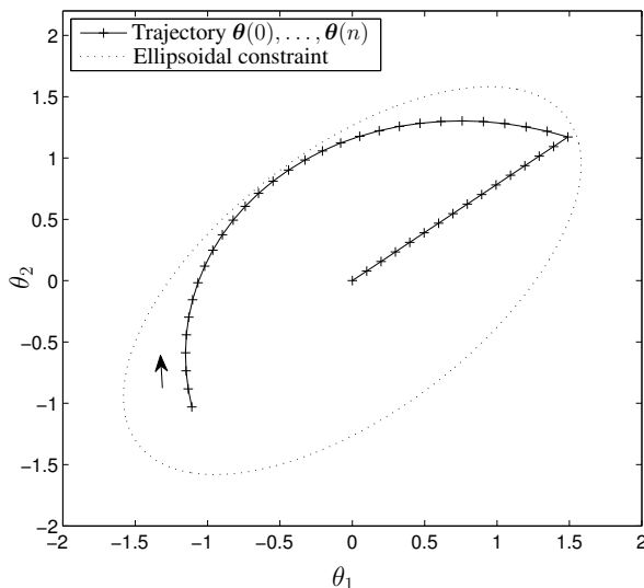
Figure 3.1: Example 1: True trajectory of \boldsymbol{\theta}(n)
