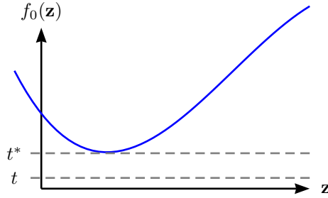
Figure C.3: Visual representation of the optimization problem (C.42)
