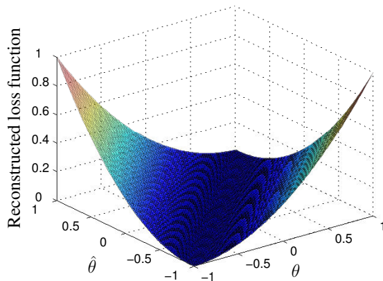
Figure 5.1: Example 1: Reconstructed loss ( D = 1 , trace and unit volume regularization)
