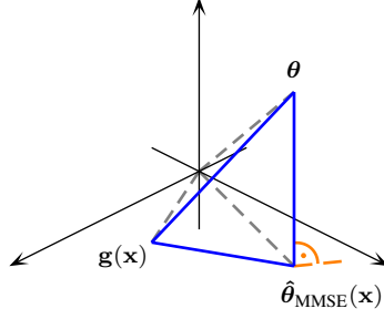
Figure C.1: Orthogonality property of the MMSE estimator
