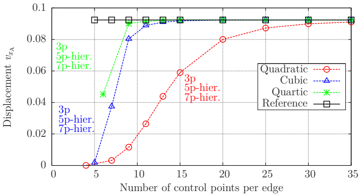
Figure 7.6: Hemisphere. Displacement convergence of “3p”, “5p-hier.”, “7p-hier.” displacement models.
