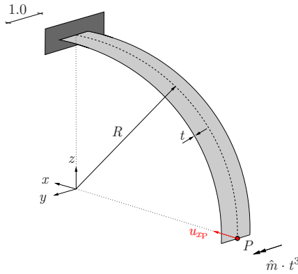
Figure 5.13: Cylindrical shell – problem setup.
