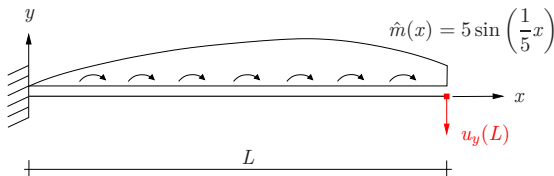
Figure 5.10: Timoshenko beam with sinusoidal moment loading.
