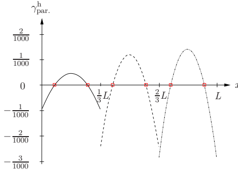
Figure 6.2: Timoshenko beam – parasitic transverse shear strains \gamma_{\text{par}}^h .
