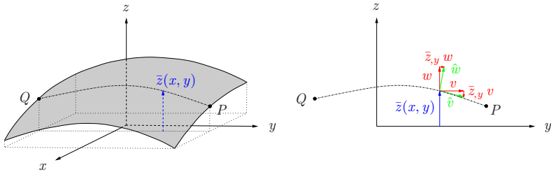
Figure 5.12: Marguerre shallow shell.
