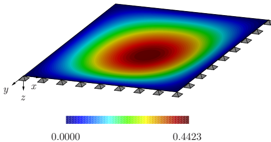
Figure 5.5: Kirchhoff-Love shell – deformation plot v_z .
