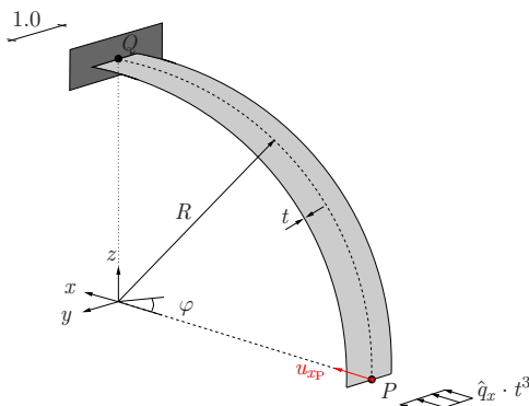
Figure 5.16: Cylindrical shell with transverse loading \hat{q}_x .
