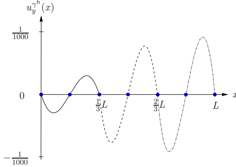
Figure 6.3: Timoshenko beam – shear gap functions u_y^{\gamma^h}(x) .
