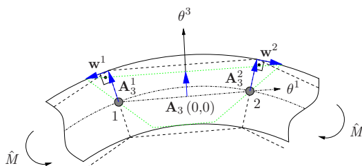
Figure 5.15: Pure bending deformation – curvature thickness locking.
