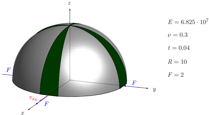
Figure 7.5: Pinched hemisphere (gray) and bending strips (green) – problem setup.
