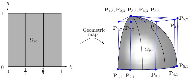
Figure 3.12: Spherical NURBS surface and bivariate basis functions.
