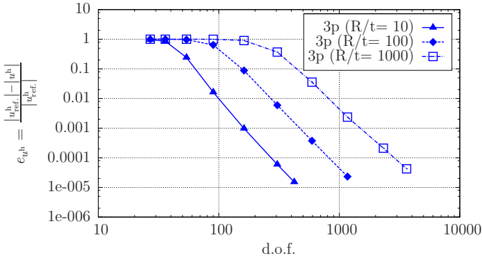
Figure 5.9: Pinched ring – relative error e_{u^h} (effect of slenderness).
