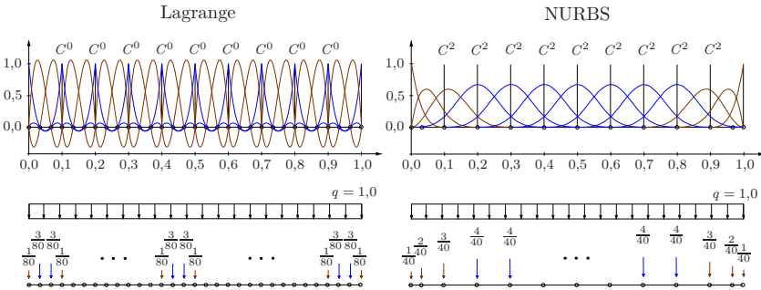
Figure 5.6: Consistent nodal forces – cubic Lagrange ( C^0 ) vs. NURBS ( C^2 ).
