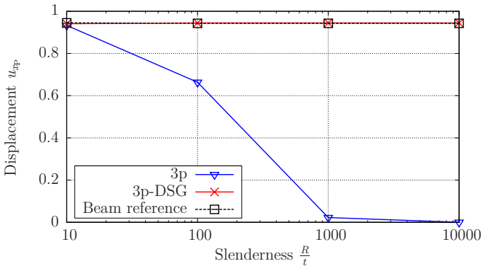
Figure 6.6: Cylindrical shell – displacement convergence, 3p shells, DSG.
