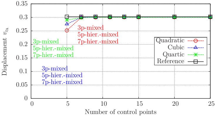
Figure 7.4: Scordelis-Lo roof. Displacement convergence of “3p-mixed”, “5p-hier.-mixed”, “7p-hier.-mixed” shell formulations.
