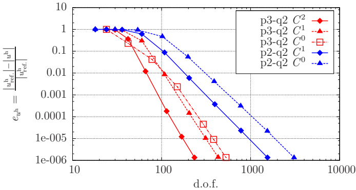
Figure 5.8: Pinched ring – relative error e_{u^h} (effect of continuity).
