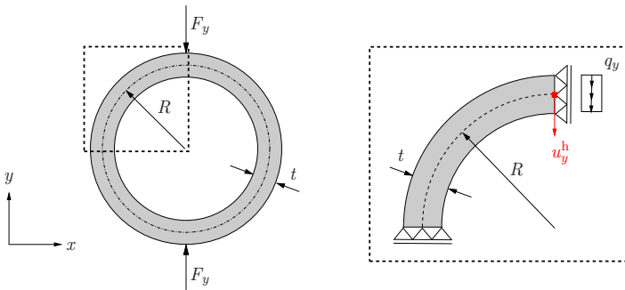
Figure 5.7: Pinched ring – problem setup.
