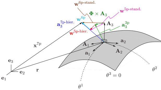
Figure 4.4: Deformed director configuration – 7-parameter models.
