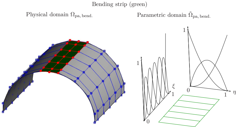
Figure 3.18: Bending strip – weak C^1 NURBS patch coupling.
