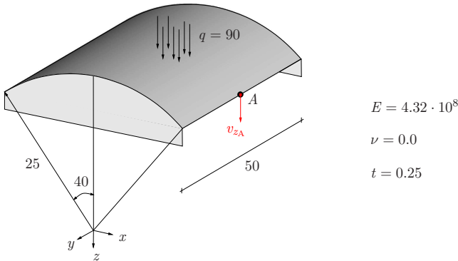
Figure 7.1: Scordelis-Lo roof – problem setup.
