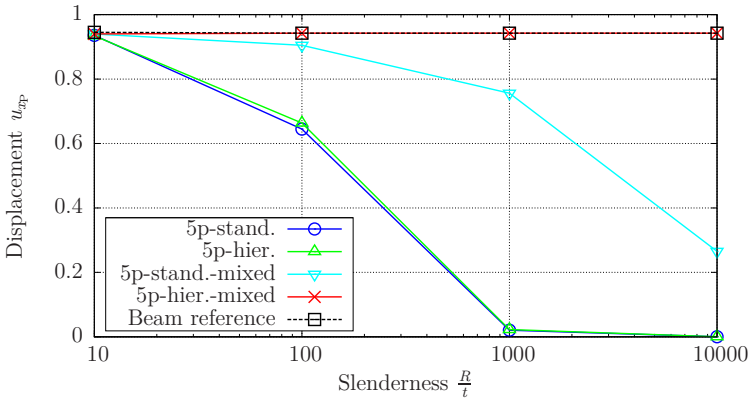
Figure 6.11: Cylindrical shell – displacement convergence, 5p shells, mixed \mathbf{u}\text{-}\boldsymbol{\sigma} .
