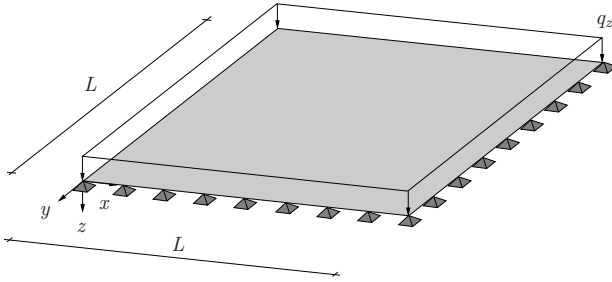
Figure 5.4: Simply supported plate with uniform transverse load.
