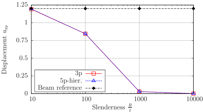
Figure 5.14: Cylindrical shell – displacement convergence (membrane locking).
