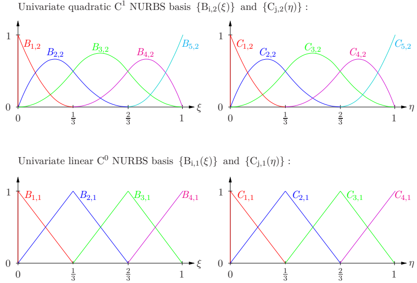
Figure 6.10: Basis functions for displacement and in-plane stress fields.
