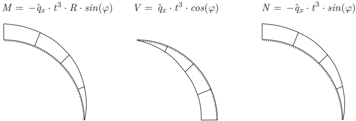
Figure 5.17: Stress resultants M, V, N – beam reference solution.
