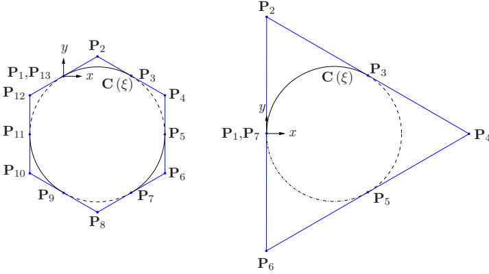
Figure 3.11: Full circles – three and six NURBS segments.
