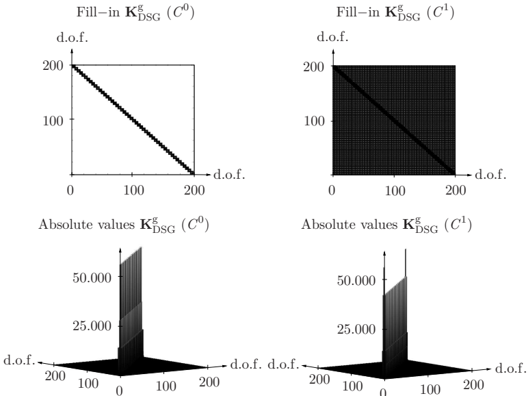
Figure 6.5: Timoshenko beam – \mathbf{K}_{\text{DSG}}^g , C^0 - vs. C^1 -continuity.
