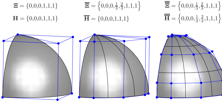
Figure 3.14: Knot refinement – spherical NURBS segments and control polygons.
