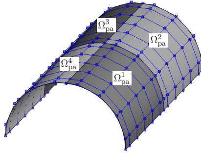
Figure 3.17: Compatible NURBS multipatch – C^0 -continuous coupling.
