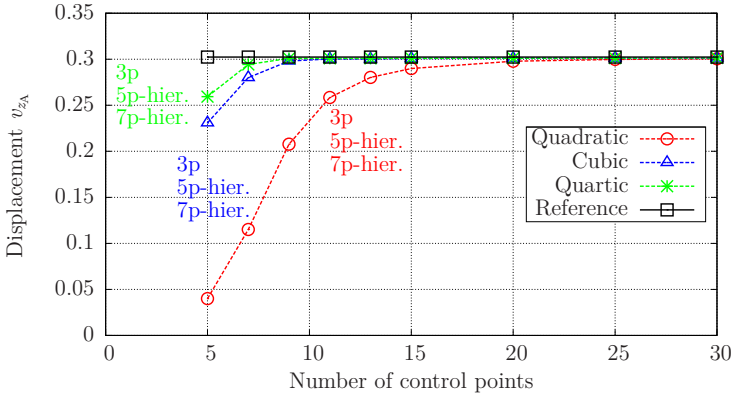
Figure 7.2: Scordelis-Lo roof. Displacement convergence of “3p”, “5p-hier.,” “7p-hier.” displacement models.
