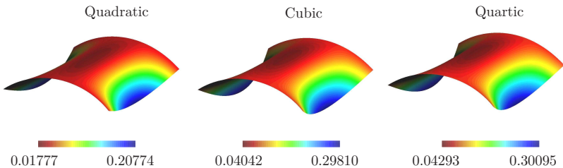
Figure 7.3: Scordelis-Lo roof. Displacement plots v_z of “5p-hier.” shell – quadratic to quartic NURBS.
