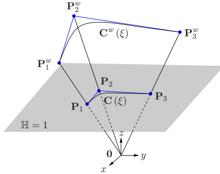
Figure 3.9: Projective transformation – generation of a NURBS curve.
