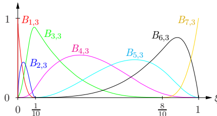
Figure 3.6: Cubic nonuniform B-spline basis \mathbf{B}_3 of \Xi_3 .
