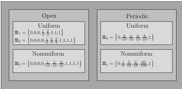
Figure 3.2: Types of knot vectors.
