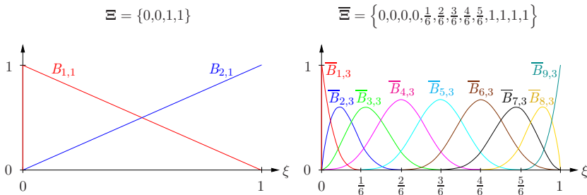
Figure 3.16: K-refinement – one-dimensional B-spline basis.
