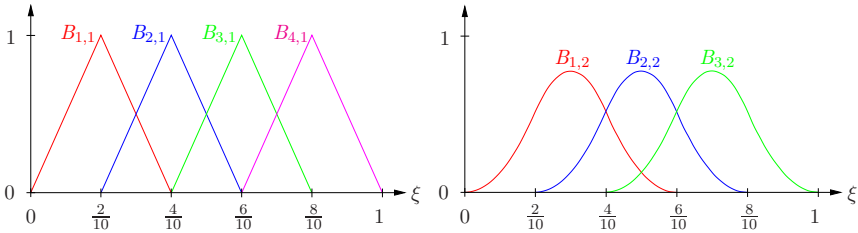
Figure 3.7: Periodic B-spline basis functions p = 1, 2 of \Xi_4 .
