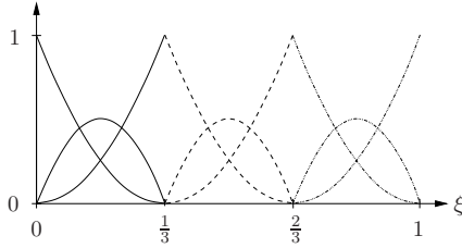
Figure 6.1: C^0 -continuous B-spline basis \mathbf{B}_2 , three elements.
