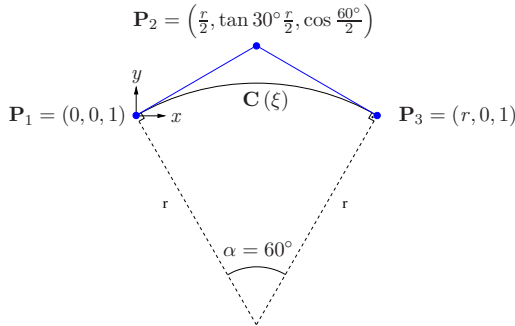
Figure 3.10: Circular arc ( \alpha = 60^\circ ) – quadratic NURBS curve.
