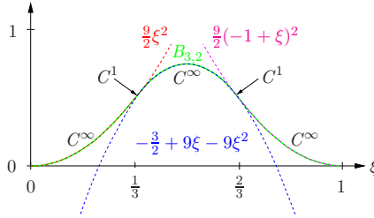
Figure 3.5: Polynomial segments of B_{3,2} .
