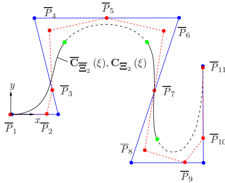
Figure 3.15: Order elevation – B-spline curve \bar{C}_{\Xi_2}(\xi) .
