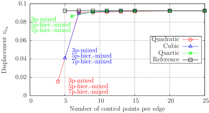
Figure 7.7: Hemisphere. Displacement convergence of “3p-mixed”, “5p-hier.-mixed”, “7p-hier.-mixed” shells.
