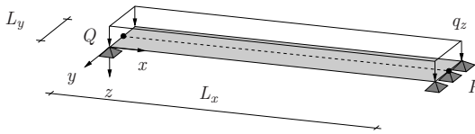
Figure 5.1: Simply supported plate strip with uniform transverse load.
