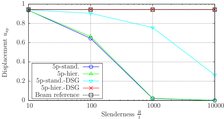
Figure 6.7: Cylindrical shell – displacement convergence, 5p shells, DSG.
