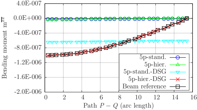
Figure 6.8: Cylindrical shell – bending moments m_{xx} , 5p shells, DSG.
