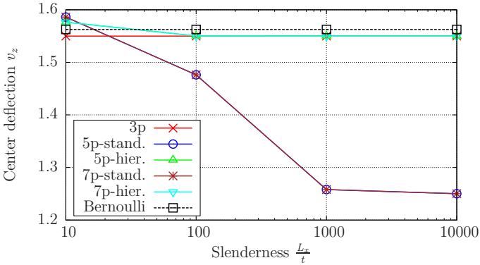
Figure 5.2: Plate strip – displacement convergence (transverse shear locking).
