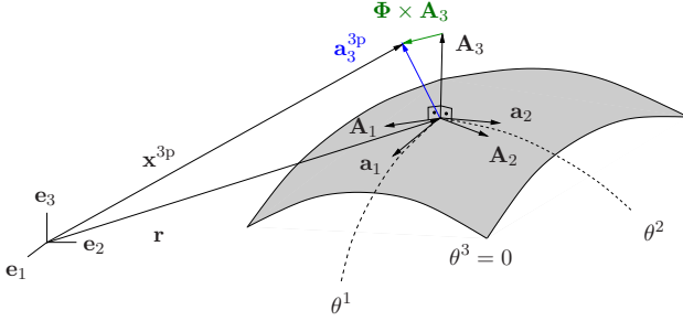
Figure 4.2: Deformed configuration – 3-parameter model.
