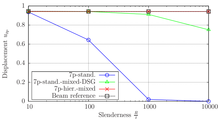
Figure 5.18: Cylindrical shell – displacement convergence (curvature thickness locking).
