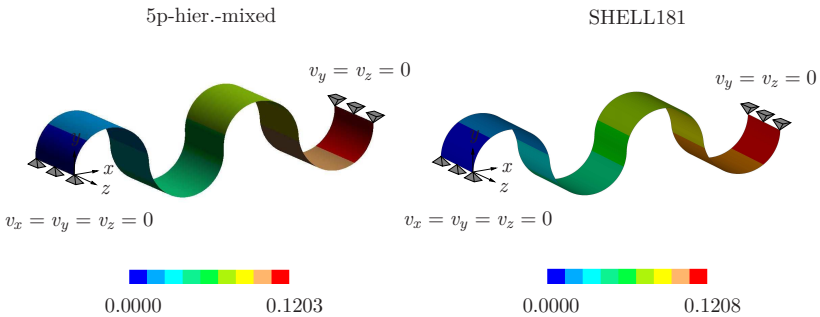
Figure 7.9: Curved shell – displacement plots v_x (5p-hier.-mixed, SHELL181).
