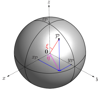
Figure 3.1: Unit sphere – types of representation.
