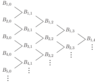
Figure 3.3: Graphical recursive relation – one-dimensional B-spline basis.
