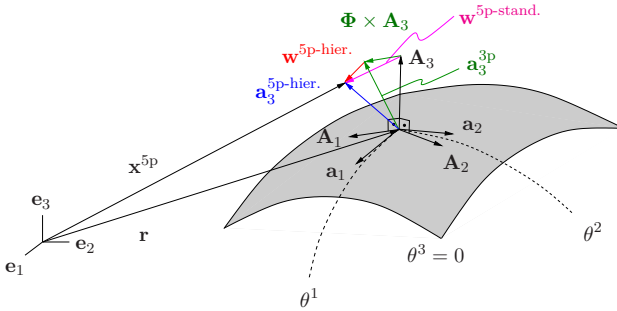
Figure 4.3: Deformed configuration – 5-parameter models.
