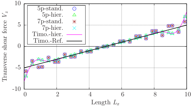
Figure 5.3: Plate strip and Timoshenko beam – transverse shear forces.
