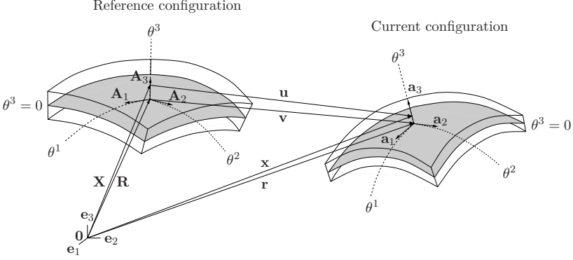
Figure 4.1: Configurations of the shell body.
