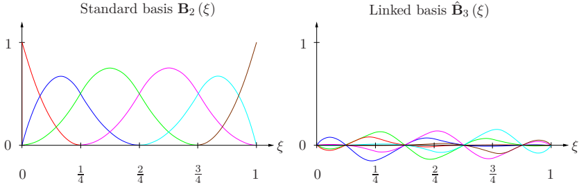
Figure 6.4: Timoshenko beam – standard and linked shape functions.
