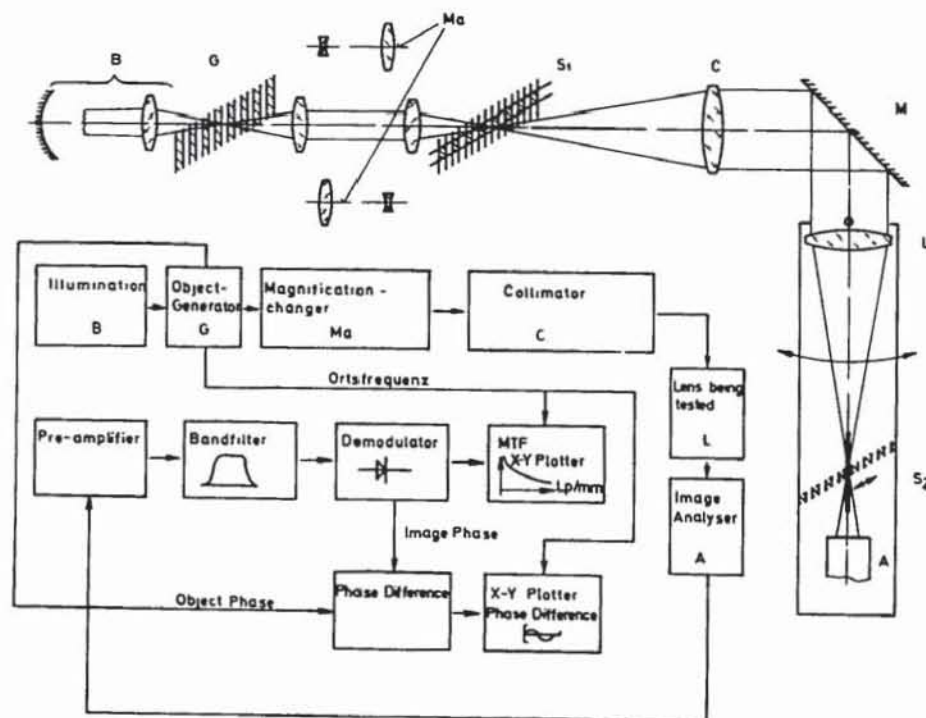
Fig.4: Principle of the equipment
