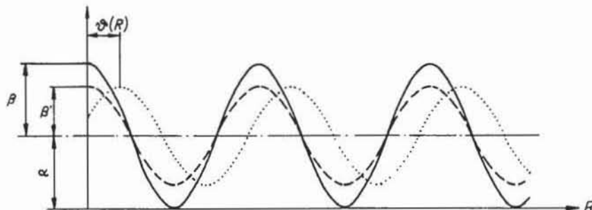
Fig.3: Principle of the optical transfer function
