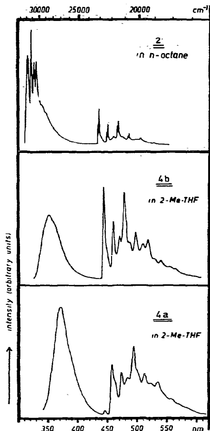
Fig. 2. Emission spectra of dimethylfluorene 2 and of syn-[2.2] (2,7) fluorenophane 4a and the anti-stereoisomer 4b in 2-methyltetrahydrofuran.
