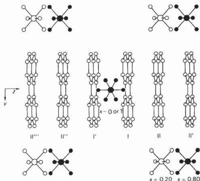
Fig. 10. Section of a stack in the 2:1 salt with surrounding PF_6^- anions, viewed along a . The centroids of perylene molecules I and II are close to x=0.50 , the shaded PF_6^- groups are above this ( x=1 or 0.80 ), the open ones below ( x=0.20 ).
