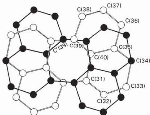
Fig. 9. The disordered perylene molecule IV in the 2:1 salt. Its centroid is at (0, 0, 1), site symmetry 2/m . Atoms C(34) and C'(34) lie on the twofold axis, the mirror plane bisects the line C(39)–C'(39).
