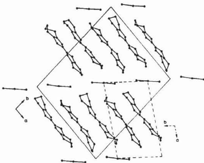
Fig. 4. \beta -(BEDT-TTF) 2 I 3 : Comparison of the low temperature supercell (solid lines) and the room temperature cell (broken lines) in a projection to the c -axis. The atom position of the low temperature structure are plotted.
