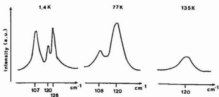
Fig. 6. Part of the Raman spectra of \beta -(BEDT-TTF) 2 I 3 at 1.4 K, 77 K and 135 K (see text).
