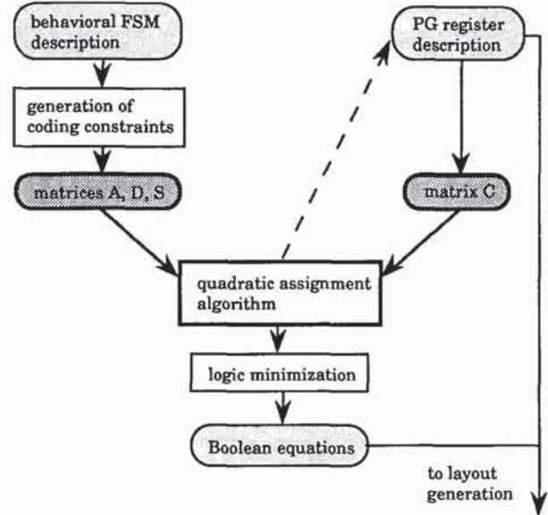
Fig. 10. Synthesis process for self-testable FSM's
