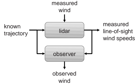
Figure 1: System theoretical view on lidar measurements and wind field reconstruction.
