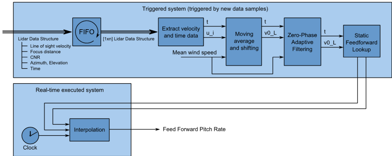
Figure 1: Schematic view of the lidar data processing for providing an estimate of the rotor effective wind speed v_{0L} to the feedforward controller.
