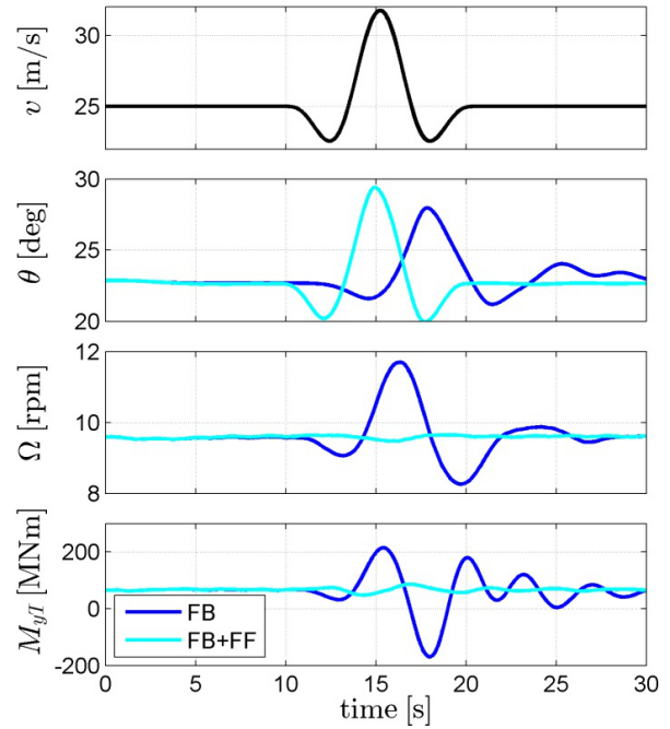
Figure 2: Response of the INNWIND.EU 10 MW wind turbine to an EOG at 25 m/s in case of perfect lidar measurement using DNV GL's Bladed .
