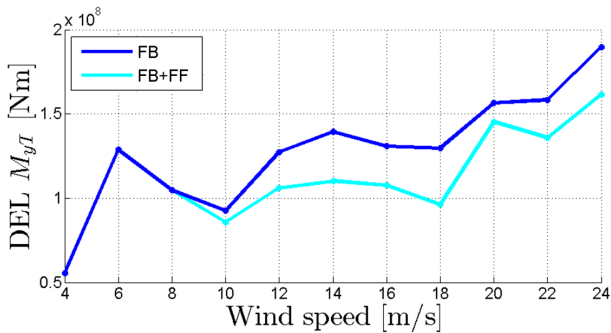
Figure 6: Lifetime-weighted DELs for the DLC 1.2 over mean wind speed.
