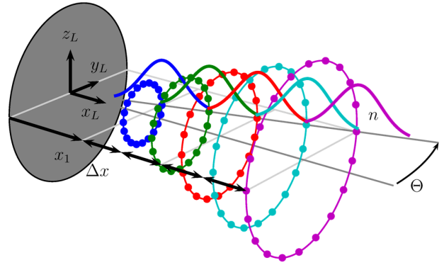
Figure 4: Visualization of an optimal scanning trajectory for the SWE-Lidar and the INNWIND.EU 10 MW wind turbine.
