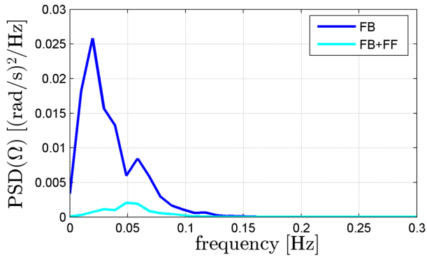
Figure 5: Power Spectral Density of a 1 h simulation at 16 m/s (Turbulence: Class A).
