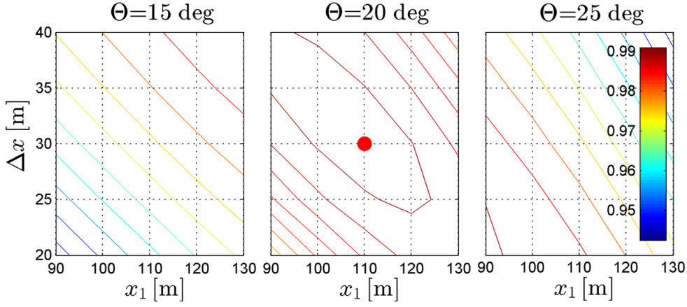
Figure 3: Optimized correlation coefficient \rho_{LR} between v_{0L} and v_0 : Optimal setup: x_1 = 110m , \Delta x = 30m , \Theta = 20^\circ .
