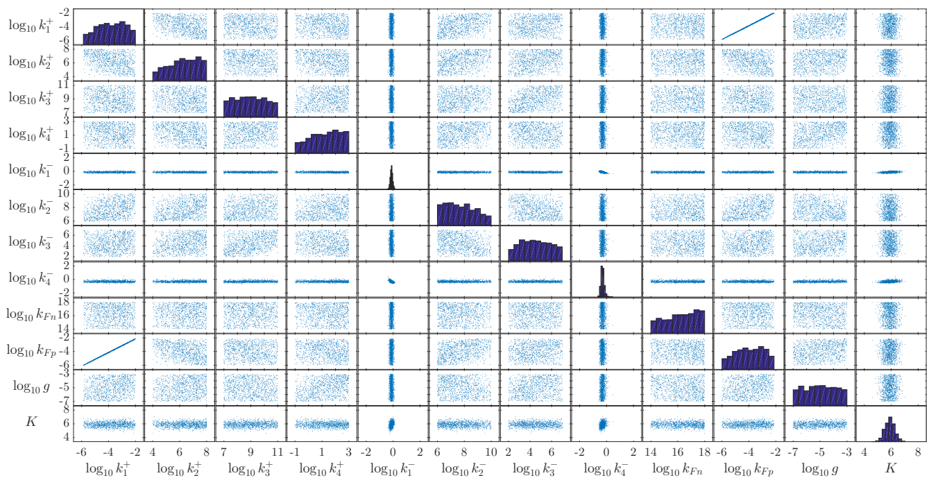
Figure 1: 2D scatter plot matrix for the parameters with histograms on the diagonal.
