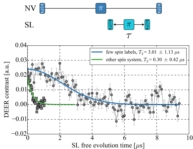
Figure 5.17.: DEER Hahn echo measurement on MTSSL spins. The blue curve is acquired on the NV-center shown in figure 5.14b, the green curve on another NV-center on the same sample, that has a different MTSSL spin configuration.
