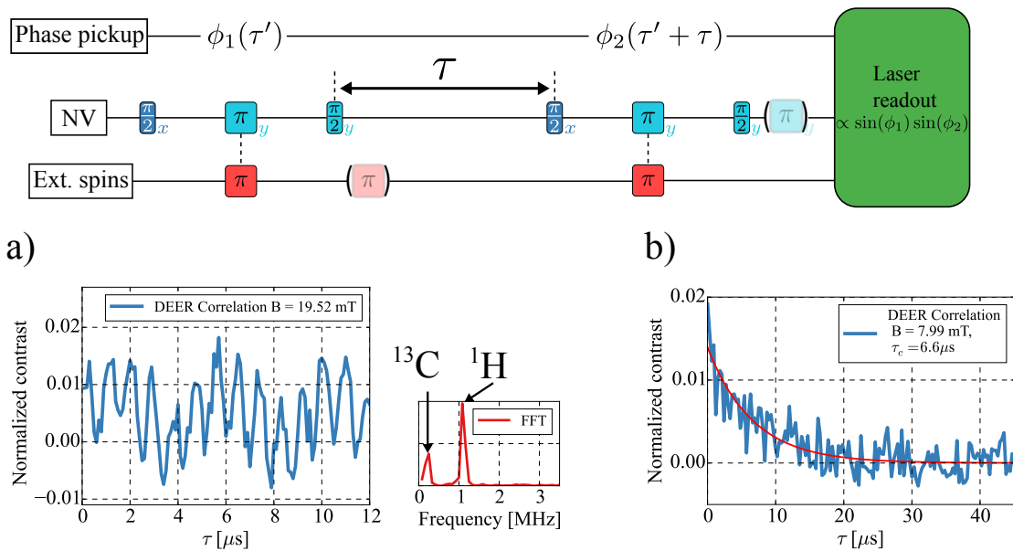
Figure 4.7.: Principle of DEER correlation spectroscopy. Two separate DEER measurements with pulses along x - and y -axes to correlate phase pickup are conducted. a) DEER correlation spectroscopy on a surface spin with long correlation time. FFT of the acquired signal to the right reveals carbon and hydrogen Larmor frequencies. b) DEER correlation spectroscopy on a different surface spin, where correlation ( T_1 ) is much shorter.
