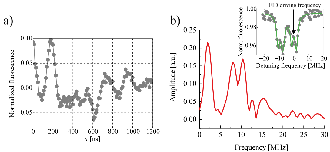
Figure 2.11.: FID measurement. a) Measurement data on a typical NV-center. The envelope yields the T_2^* time, usually below 1 \mu\text{s} for shallow implanted NV-centers. b) FFT of the measured signal. We can distinguish couplings that most likely stem from the closeby ^{15}\text{N} nuclear spin and a weakly coupled ^{13}\text{C} spin.
