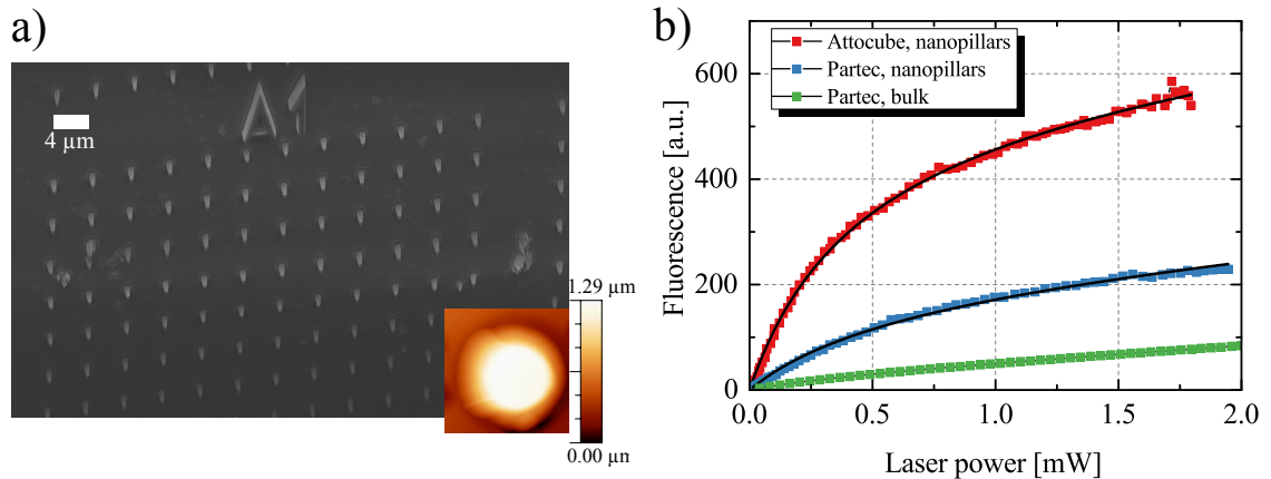
Figure 3.2.: Increasing NV-center fluorescence collection efficiency at low temperatures. a) SEM image of a nanofabricated diamond nanopillar membrane. Inset shows an ambient AFM scan over a single pillar. b) Comparison of bulk and nanopillar diamond samples and Partec or Attocube microscope objectives at low temperature on the same NV-center.
