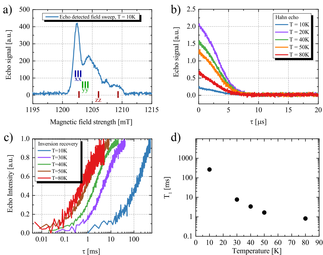
Figure 5.4.: Pulsed EPR on MTSSL labeled NP 10 N peptides at low temperatures in D 2 O/glycerol (4:1) solution. a) Echo detected field sweep at T = 10 K and Q-band frequency. The different hyperfine components are indicated in the graph. b) Hahn echo measurements over a temperature range, yielding the coherence time T_2 of the measured spin species. Transverse relaxation time is unaffected in the shown temperature range. c) Saturation recovery measurements, that yield the longitudinal relaxation time T_1 . d) Plot of single exponential fits to the measurement data of c).
