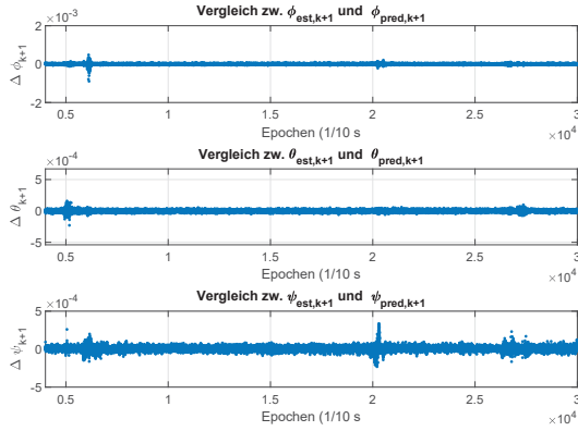
(a) \Delta\Theta_{k+1}
