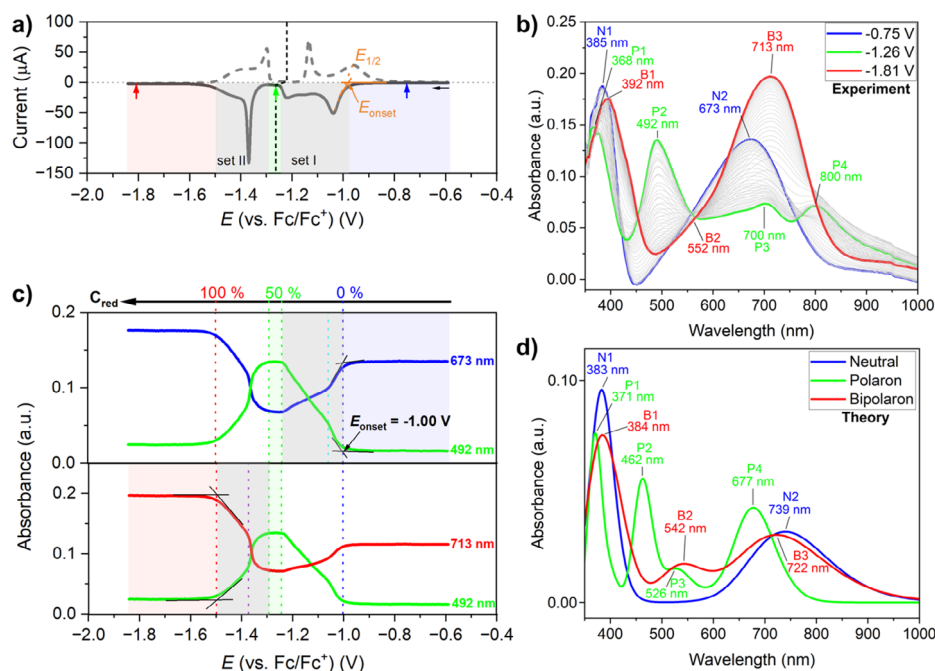
Figure 2. a–c) In situ spectroelectrochemistry measurements of a spin-coated film of P(NDI2OD-T2) on an ITO glass substrate upon reduction, scan rate 20 mV s −1 in 0.1 M TBAPF 6 /acetonitrile electrolyte. (a) Second cycle of reduction. (b) UV–vis absorption spectra recorded in situ during the forward scan. The characteristic spectra for the neutral (N), polaron (P), and bipolaron (B) states of P(NDI2OD-T2) are indicated by blue (N1, N2), green (P1, P2, P3, P4), and red (B1, B2, B3) spectra. (c) Spectral evolutions of characteristic peaks at 673 nm (N2), at 492 nm (P2), and at 713 nm (B3) are plotted as function of potential during the forward scan. The blue, green, and red shading indicate the potential ranges of the fully neutral, fully polaron, and fully bipolaron states, respectively. The gray shading refers to the potential ranges for the transition from the neutral to polaron (set I) and from polaron to bipolaron states (set II), i.e., potential ranges for mixed charged species. d) TD-DFT calculated UV–vis absorption spectra of neutral and charged states of an NDI-T2 dimer are shown.
